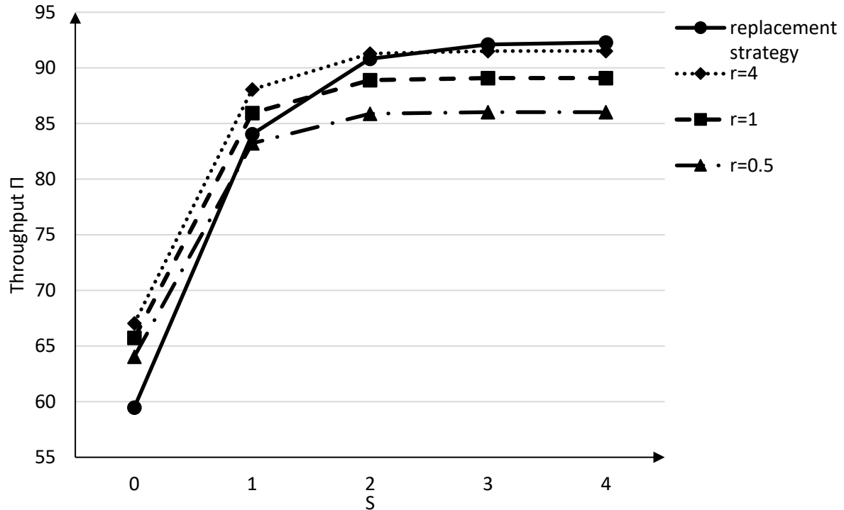
Figure 2 Impact of repair rate on throughput
