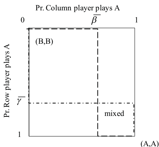
FIGURE 2: Best-response Correspondence
