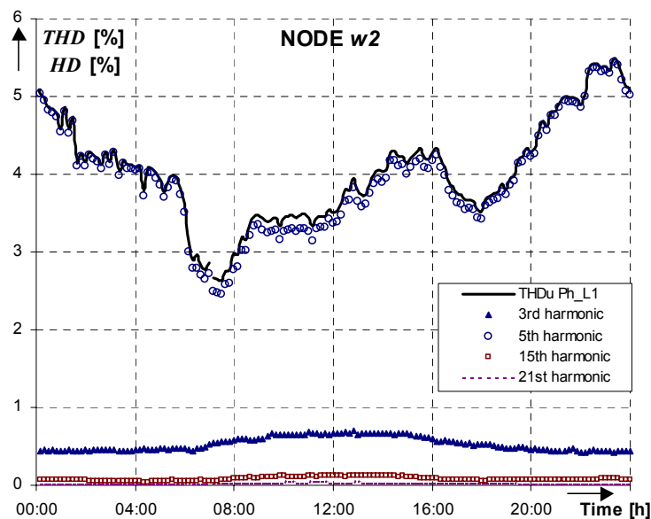
Fig. 5.9 THD and HD factors at node w2
