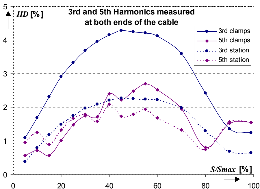
Fig. 4.7 Harmonic content of the voltage measured at the clamps (a) and station (A)
