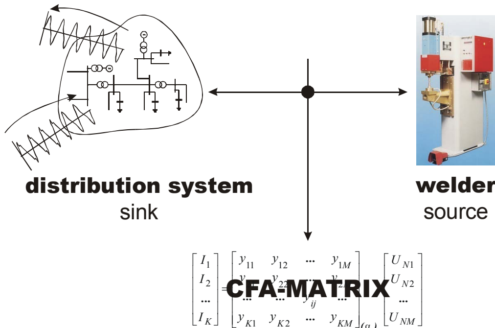
Fig. 4.10 Coupling representation for distribution network (sink for disturbance) – load (source of disturbance)
