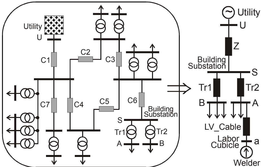
Fig. 4.4 The system and its simplification modeled for the welder case study
