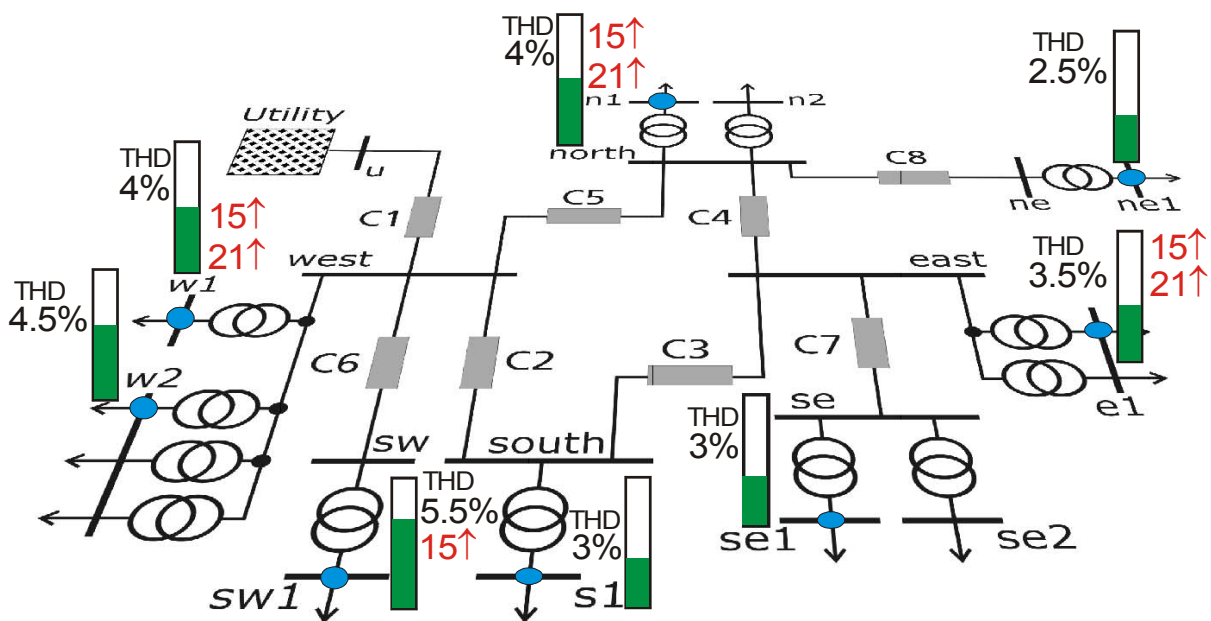
Fig. 5.5 THD level within the distribution network
