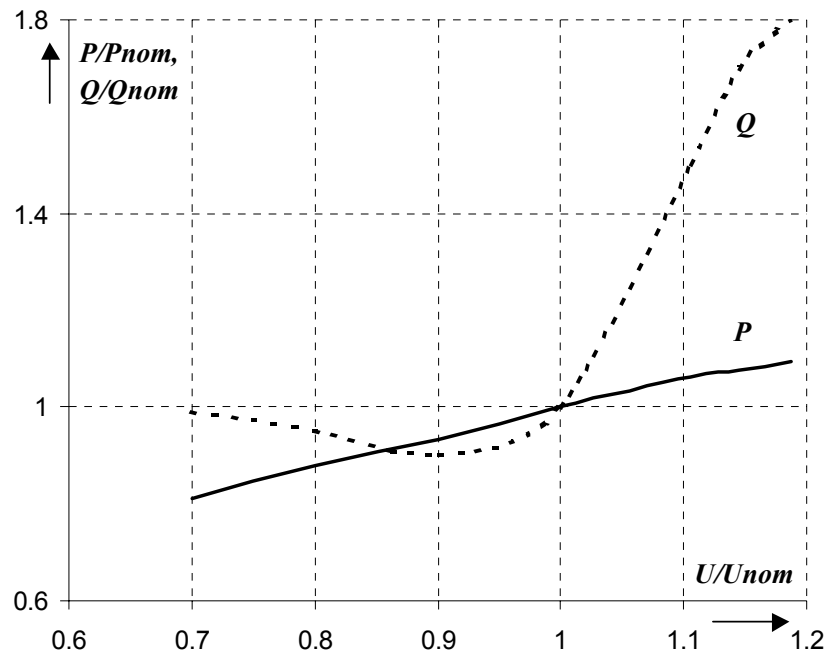
Fig. 5.21 Modeling of the load with non-linear P, Q = f(U) characteristic
