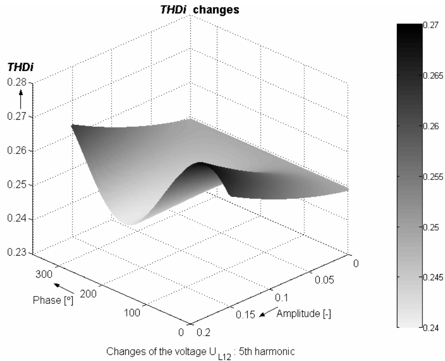
Fig. 4.17 Influence of the 5 th harmonic voltage U_{L12} changes on the THDi of the current drawn by the machine
