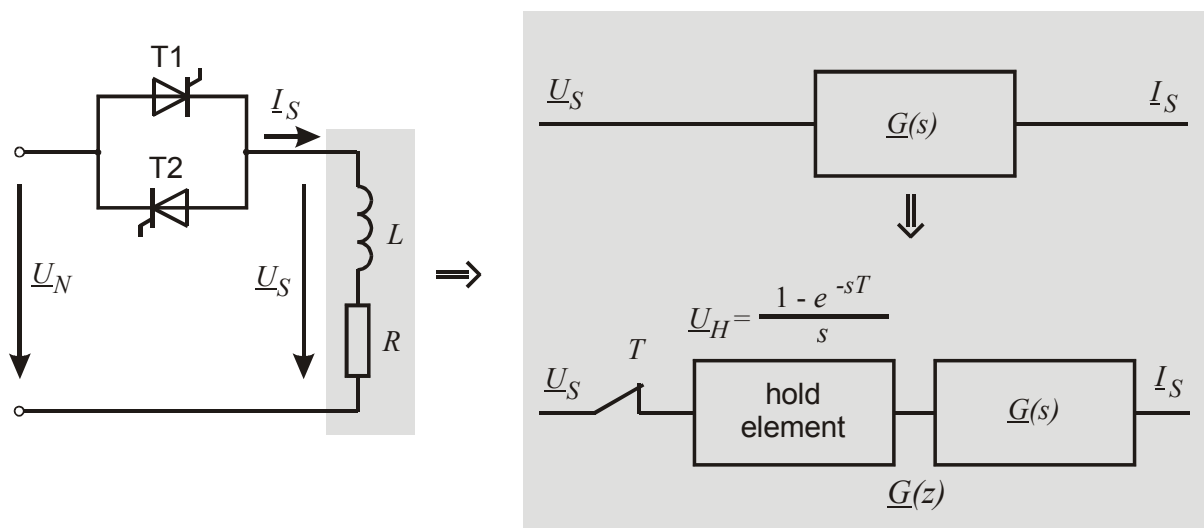
Fig. 4.13 Parameterization of the welding machine and transmittance based procedure for the measurement-based parameter identification
