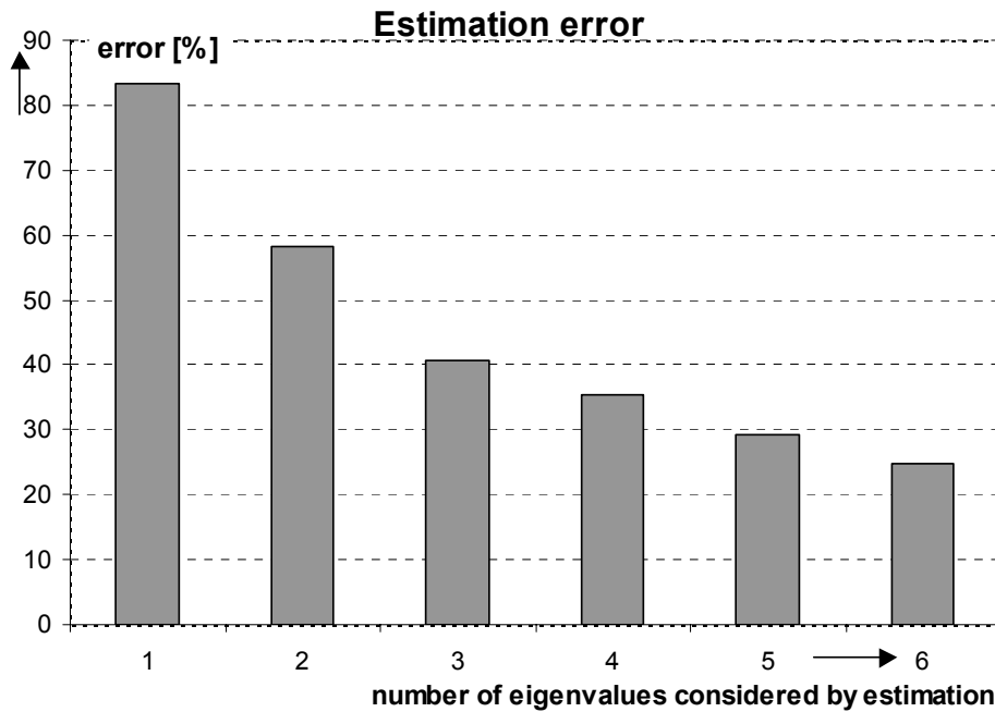
Fig. 5.19 Estimation error for the quantitative analysis, 15 th harmonic case
