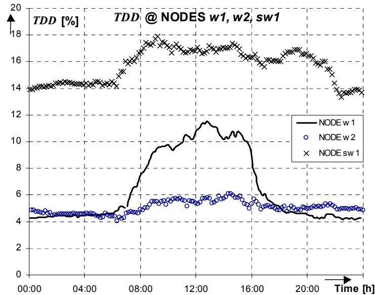
Fig. 5.8 TDD of the currents measured at node w1 , w2 and sw1
