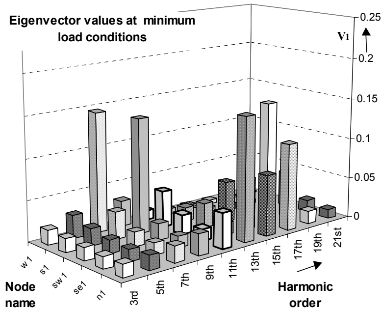
Fig. 5.22 Eigenvector values, which correspond to the minimum eigenvalue at minimum load conditions
