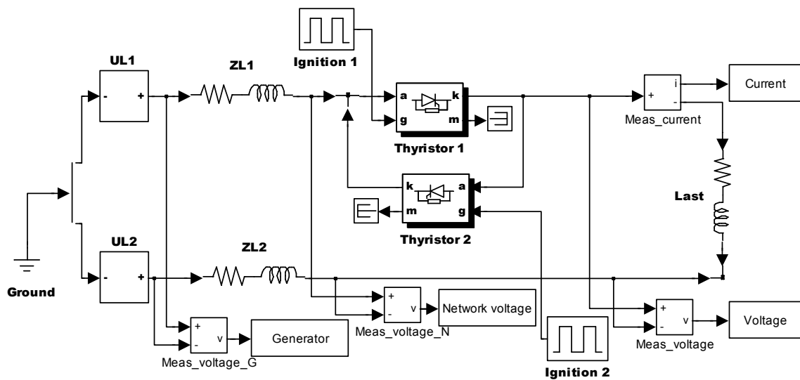
Fig. 4.16 Model of the welding machine with the identified parameters and network impedance
