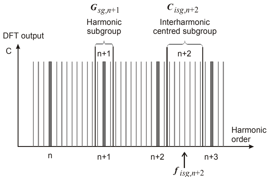
Fig. 3.5 Grouping of DFT-bins into the harmonics and interharmonics subgroups [46]
