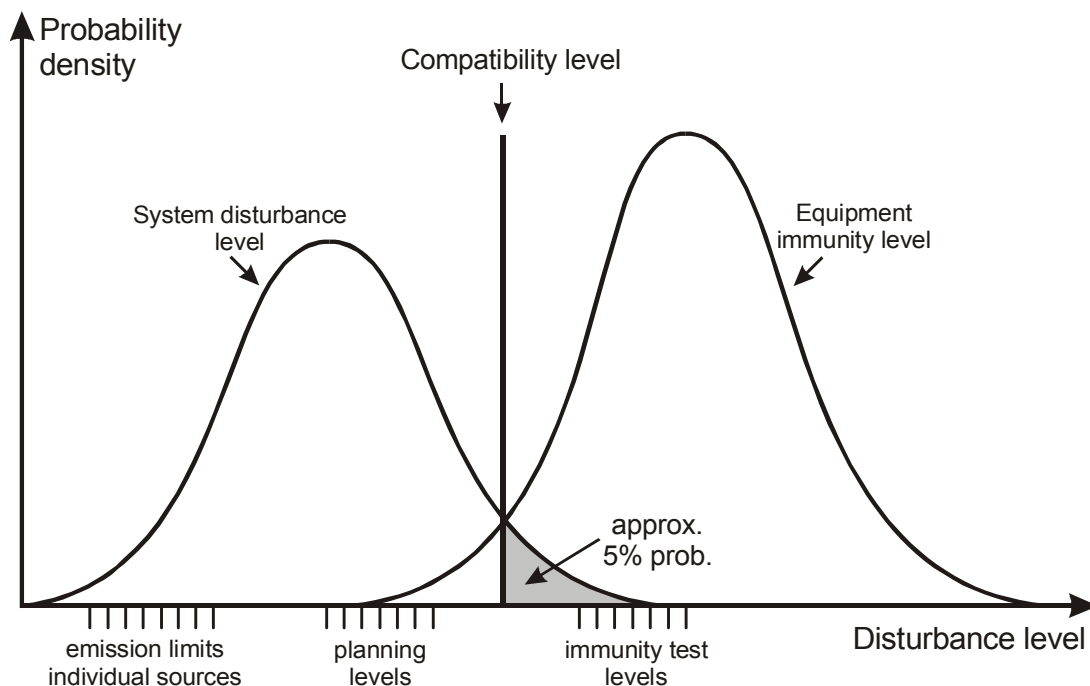
Fig. 2.2 General concept of the electromagnetic compatibility in electrical power networks [26]
