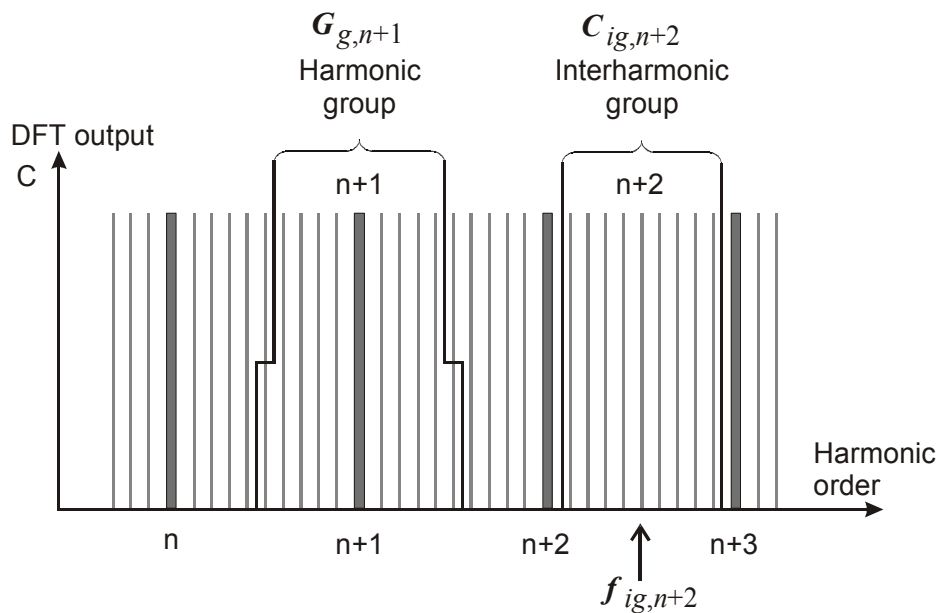
Fig. 3.4 Grouping of DFT-bins into the harmonics and interharmonics groups [46]
