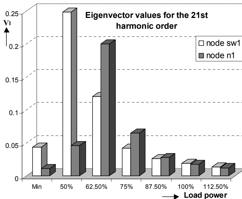
Fig. 5.25 Eigenvector values changes as a function of the non-linear load power calculated for 21 st harmonic order
