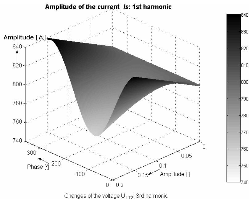
Fig. 4.19 Influence of the 3 rd harmonic voltage U_{L12} changes on the first harmonic current drawn by the machine
