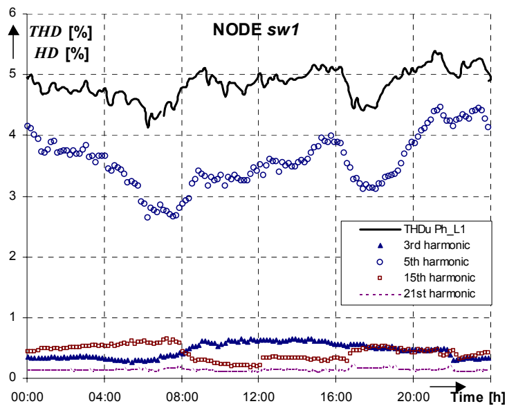
Fig. 5.10 THD and HD factors at node sw1
