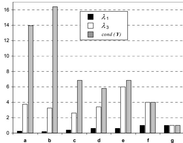
Fig. 5.2 Minimal ( \lambda_1 ) and maximal ( \lambda_3 ) eigenvalues and the conditionality number ( cond(Y) ) calculated for the network configurations from Fig. 5.1
