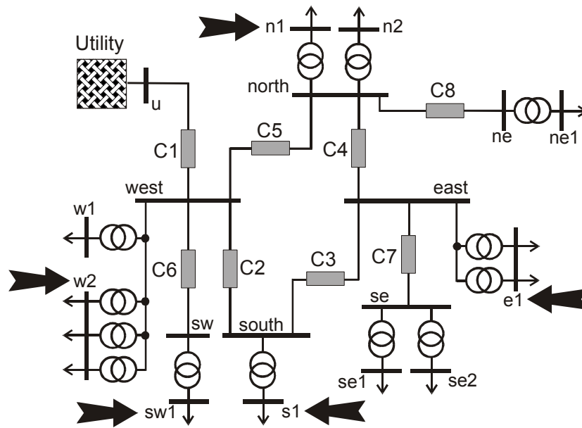
Fig. 5.17 Distribution system with the most considerable nodes to which attention should be paid in cases of unbalance for characteristic and non-characteristic harmonics
