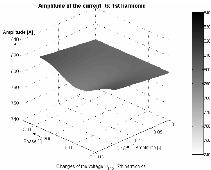
Fig. 4.20 Influence of the 7 th harmonic voltage U_{L12} changes on the first harmonic current drawn by the machine
