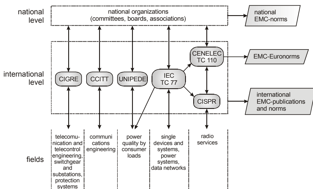
Fig. 2.3 Important institutions responsible for the development of standards in EMC [21]
