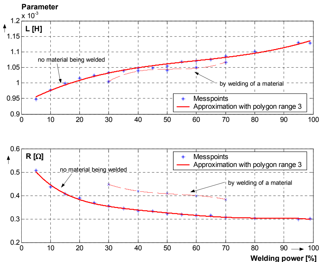
Fig. 4.14 Parameter L and R identified as a function of the welding power, for the short circuit welding condition and during the welding process of a metal plate
