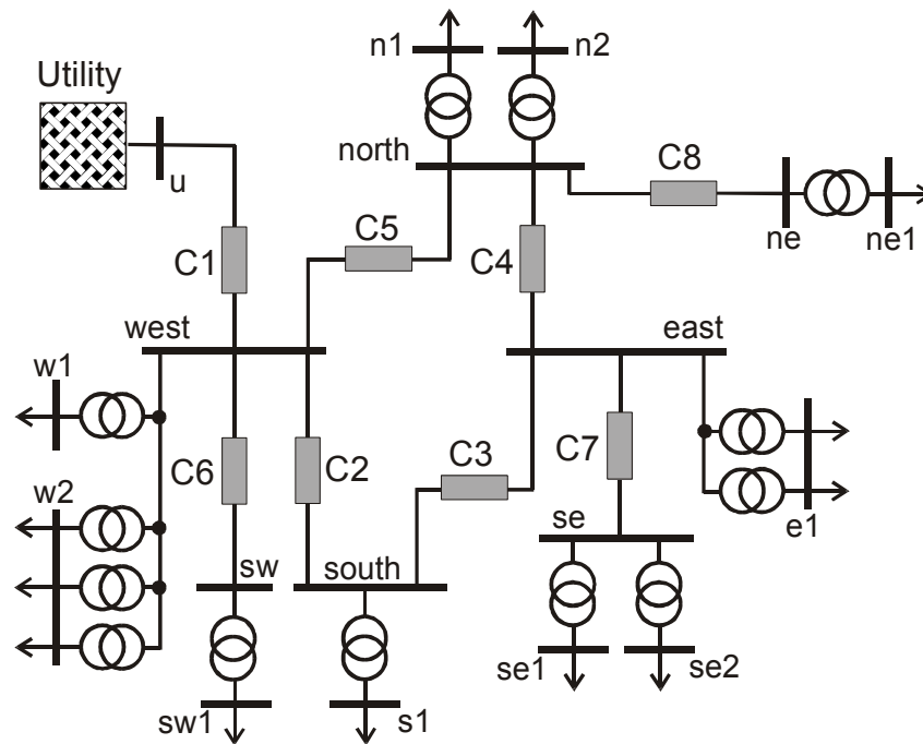
Fig. 5.4 Simplified test network scheme
