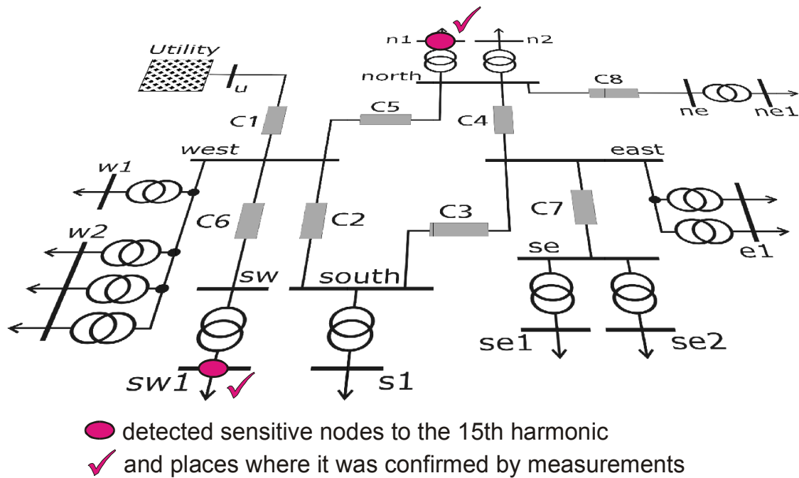
Fig. 5.18 Comparison measurements – sensitivity analysis, 15 th harmonic case
