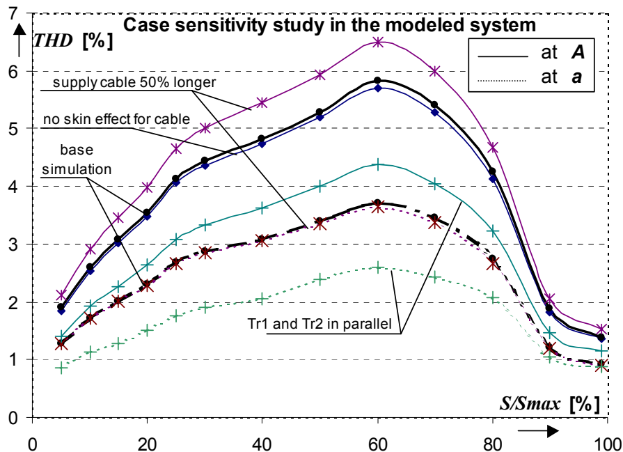
Fig. 4.9 Influence of the model parameter on the harmonic distortion at the clamps (a) and at the bus (A)
