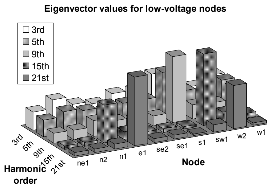
Fig. 5.16 Eigenvector values for the minimum eigenvalue calculated for low-voltage nodes in the studied system at chosen harmonic orders
