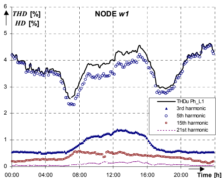
Fig. 5.6 THD and HD factors at node w1 for phase L1
