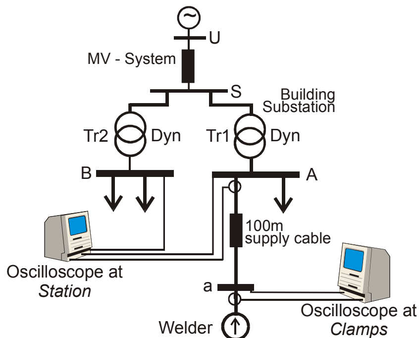
Fig. 4.6 Measurement setup in the studied distribution system
