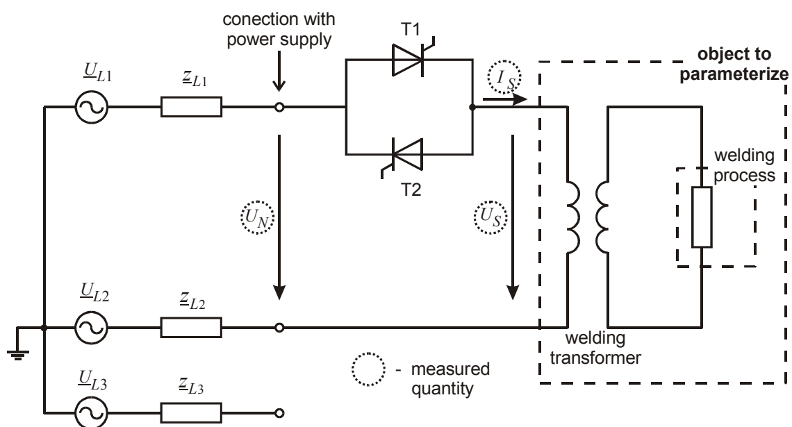
Fig. 4.12 Measuring arrangement for the identification of the welding process' parameters
