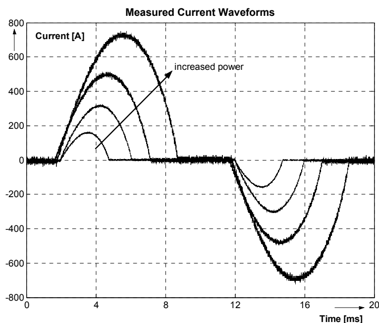
Fig. 4.3 Waveforms of the current demanded by the welder by distinct welding power
