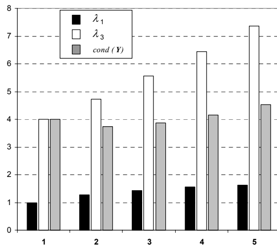
Fig. 5.3 Minimal ( \lambda_1 ) and maximal ( \lambda_3 ) eigenvalues and the conditionality number ( cond(Y) ) calculated for the different admittances of the branch 1-4 for the circuit from Fig. 5.1 f
