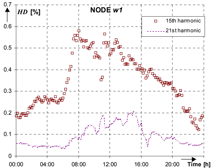
Fig. 5.7 HD factors for 15 th and 21 st harmonic orders at node w1
