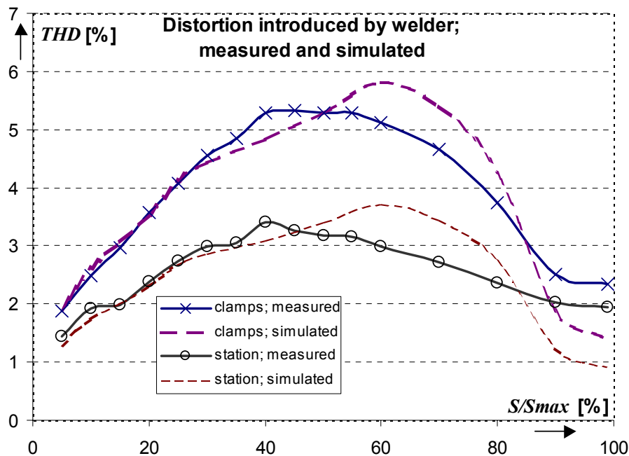
Fig. 4.8 Comparison between measurements and simulation results: Voltage distortion at both ends of the supply cable (points A, a in Fig. 4.6)
