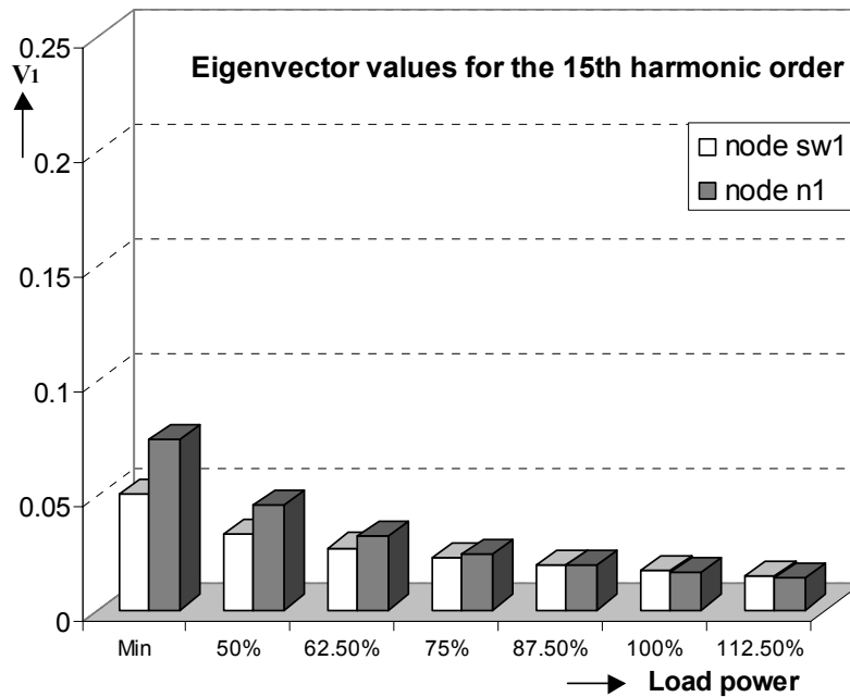
Fig. 5.24 Eigenvector values changes as a function of the non-linear load power calculated for 15 th harmonic order
