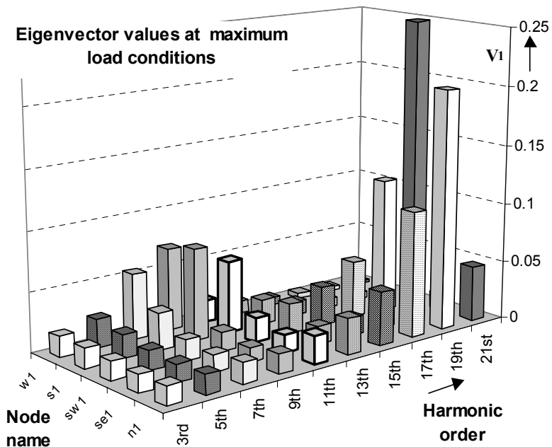
Fig. 5.23 Eigenvector values, which correspond to the minimum eigenvalue at maximum load conditions
