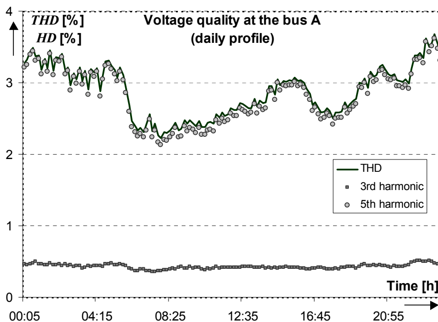
Fig. 4.5 Daily voltage quality profile at the bus A (no welder present)
