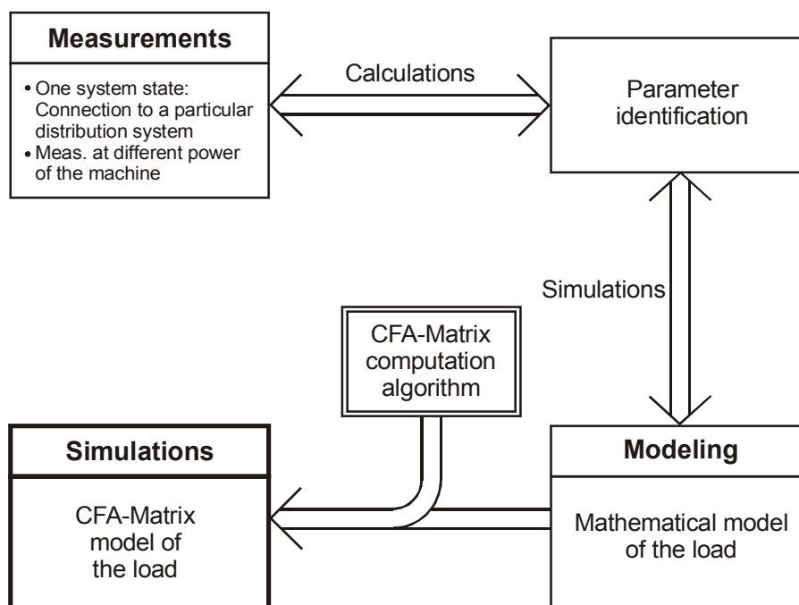
Fig. 4.11 The algorithm of the CFA- Matrix constructing process used for high power non-linear load representation
