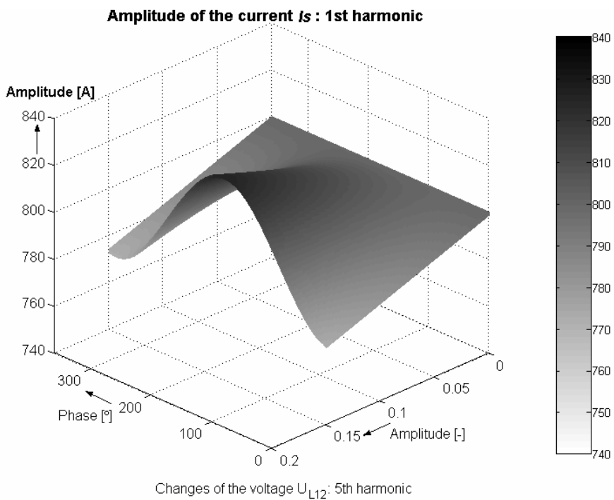
Fig. 4.18 Influence of the 5 th harmonic voltage U_{L12} changes on the first harmonic current drawn by the machine
