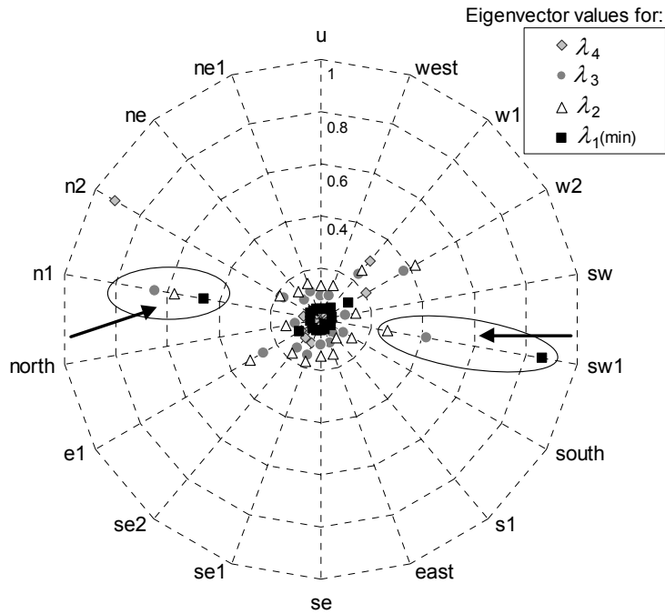
Fig. 5.20 Eigenvector values that correspond to the four smallest eigenvalues, analysis for 15 th harmonics
