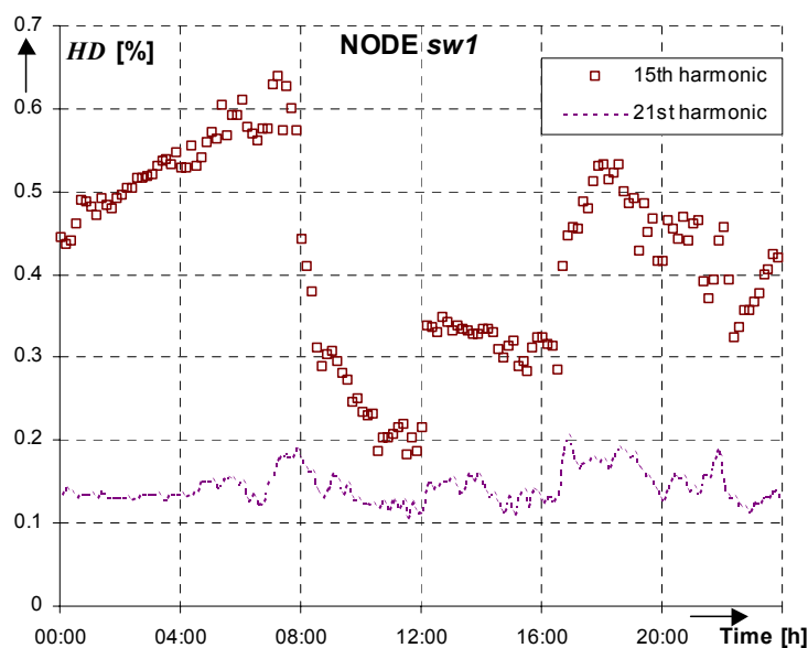
Fig. 5.11 HD factors for 15 th and 21 st harmonics at node sw1
