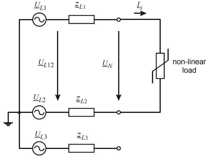
Fig. 4.15 The nonlinear load modeled with the impedance of a distribution network
