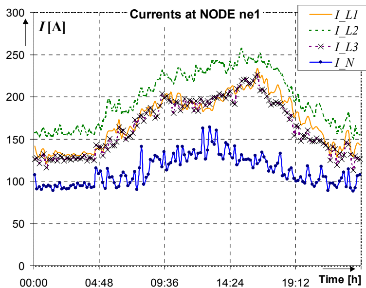
Fig. 5.12 Amplitude changes of the currents measured at bus ne1 over 24 hours
