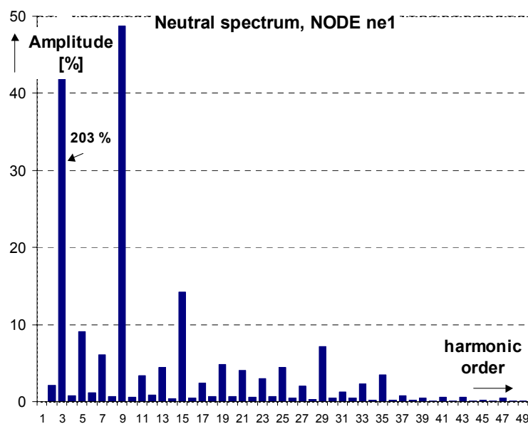
Fig. 5.13 Spectrum of the current flowing in neutral conductor at node ne1
