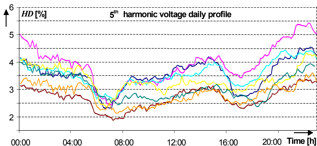
Fig. 5.15 Level of the 5 th harmonic at every site
