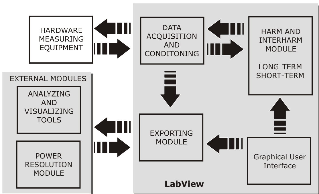
Fig. 3.1 Power quality monitoring system - general scheme
