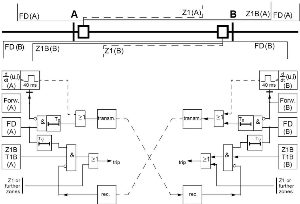
Figure 4-17- Blocking with Overreach Zone Z1B [36].
