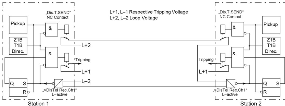
Figure 4-18- Pilot Wire Comparison [36].
