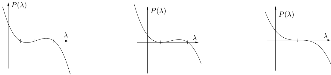
Figure 1: Curves of characteristic polynomials in the case of single and multiple eigenvalues (for positive definite tensors)
